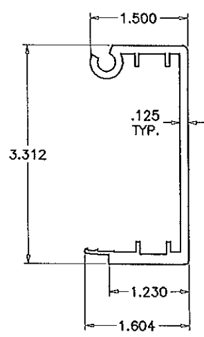
⑤ MALE POST
