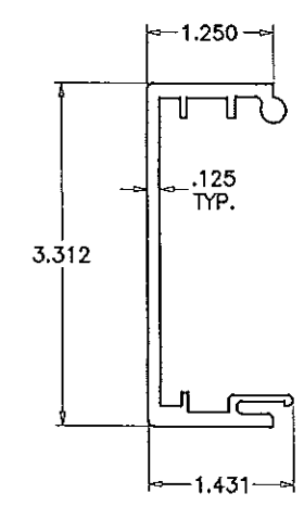
④ FEMALE POST
