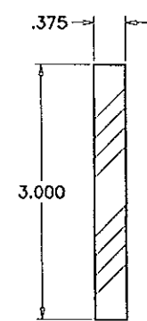
⑦ EXTERIOR GLAZING GASKET SCALE 1:1
