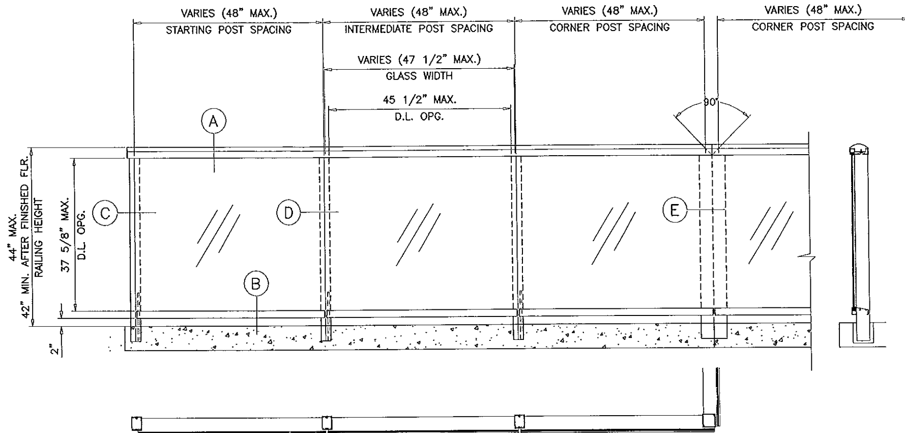
TYPICAL ELEVATION
