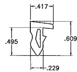
⑧ INTERIOR GLAZING GASKET SCALE 1:1
