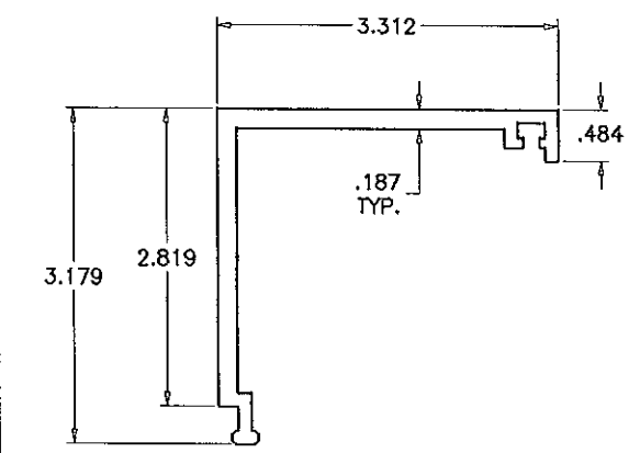
⑥ CORNER POST
