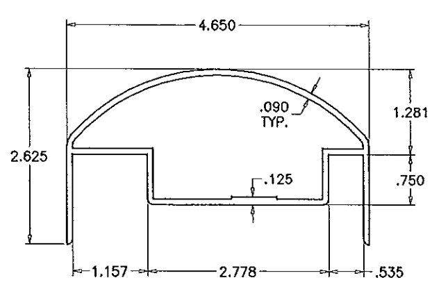
① TOP RAIL CAP
