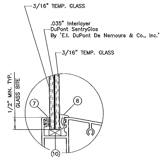
GLASS DETAIL 7/16" OVERALL LAM. GLASS
