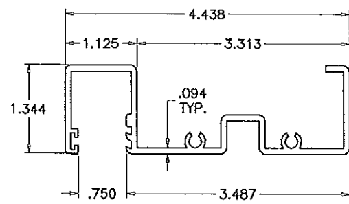
② TOP RAIL CHANNEL
