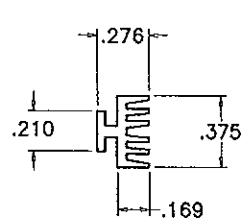
⑦ EXTERIOR GLAZING GASKET SCALE 1:1
